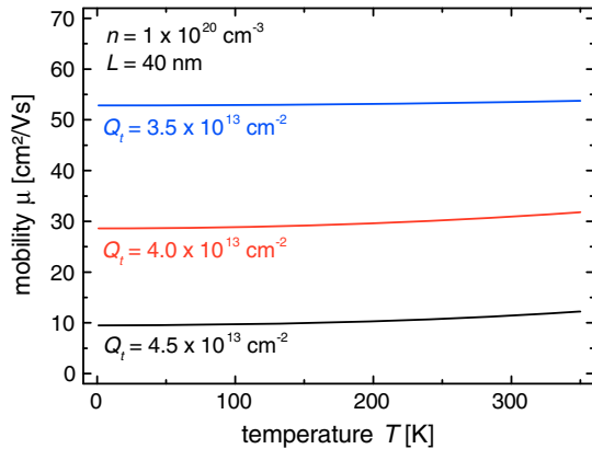
FIG. 3. The temperature-dependent mobility \mu is plotted for three different trap densities Q_t . A constant carrier concentration of 1 \times 10^{20} \text{ cm}^{-3} and a grain size of 40 nm are assumed. The mobility is almost constant for temperatures up to 100 K and increases approximately quadratic for higher temperatures. Note that the trap density influences predominantly the overall level of the mobility and not so much the general shape of the curve.
