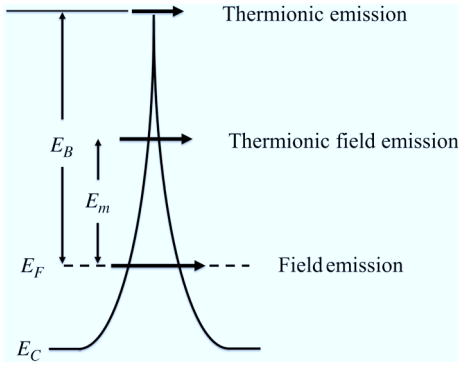
FIG. 2. A potential barrier at a grain boundary in degenerate semiconductors is illustrated. E_C and E_F denote the energy level of the conduction band and the Fermi level, respectively. The Fermi level lies within the conduction band. E_B measures the barrier height from the Fermi level to the top of the barrier. Electrons can pass the potential barrier by thermionic emission over the barrier, by thermally activated tunneling (thermionic field emission) at the energy E_m , and by tunneling (field emission) at the Fermi level.
